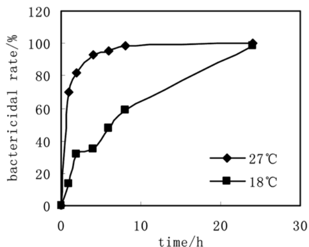
Fig. 4. The influence of temperature on the antibacterial efficiency. ( E. coli 170 rpm/min)
